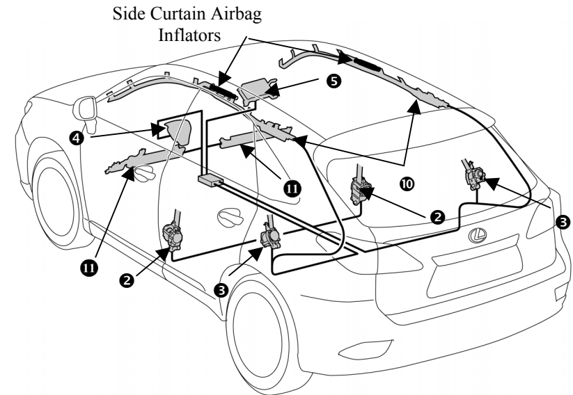
Standard Frontal Airbags, Seat Belt Pretensioners, Knee Airbag, Side Curtain Airbags
