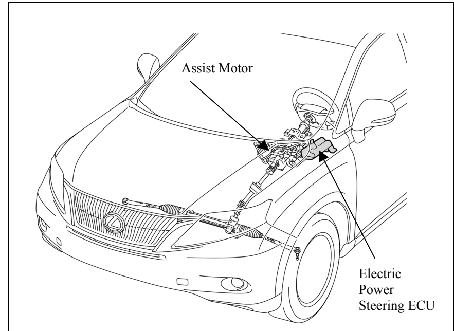
46 Volt Electric Power Steering System
