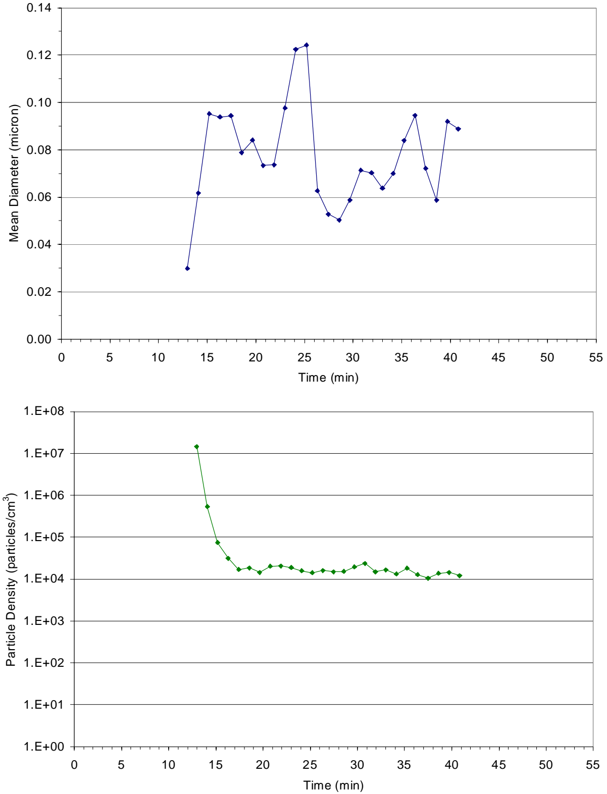
Figure 4-20: Smoke particle average size (top) and count density (bottom) measured with the particle analyzer during overhaul of the living room fire.
