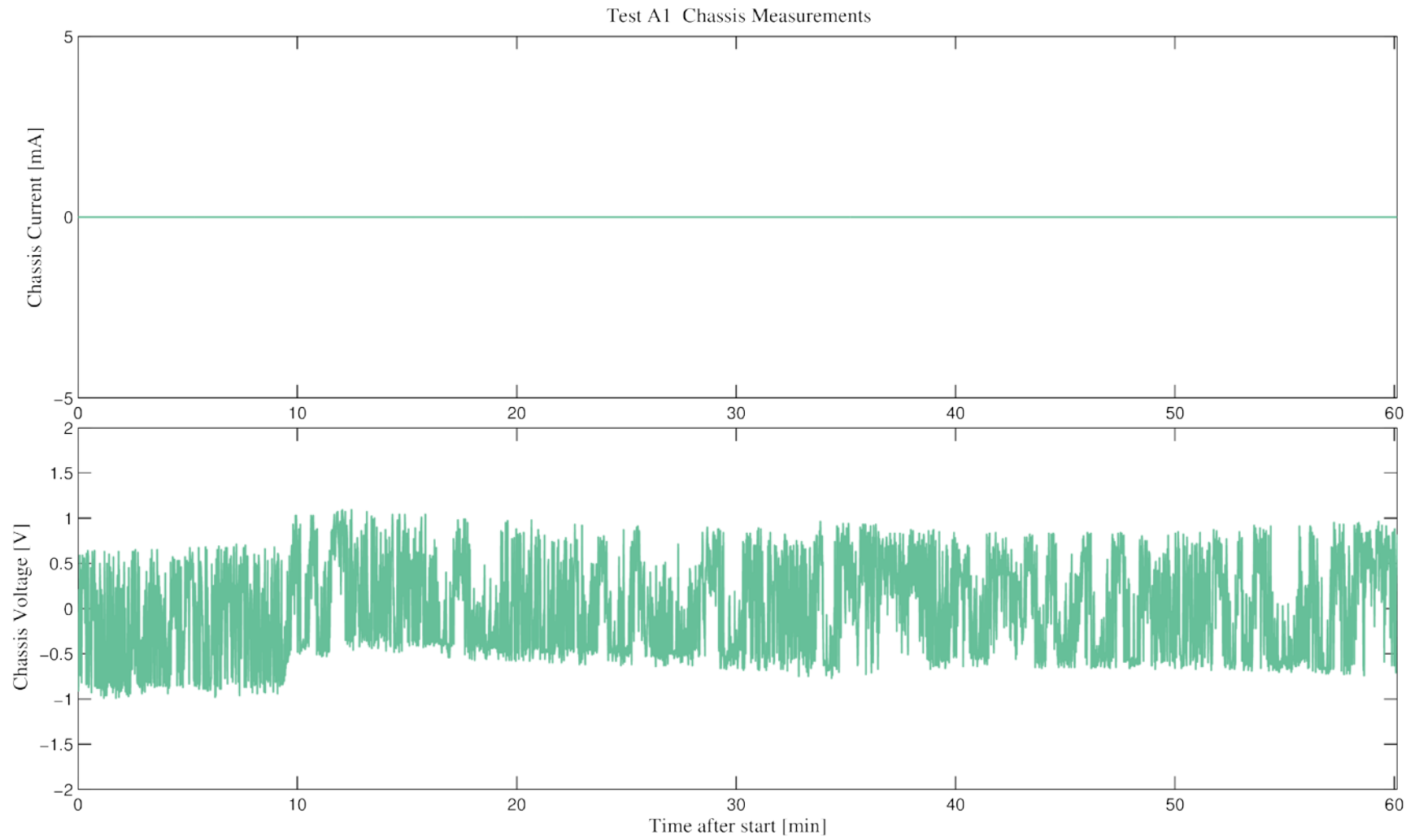
Figure E.9 Chassis voltage and current measurements for Test A1
