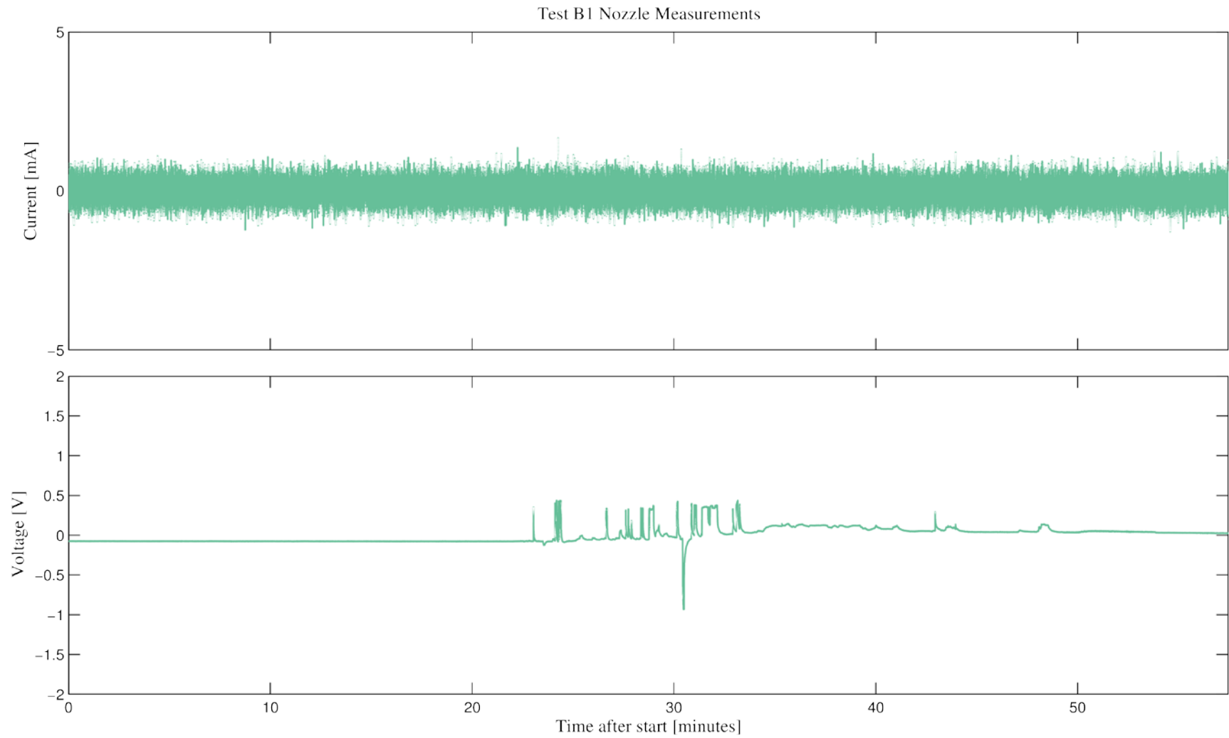
Figure E.6 Nozzle voltage and current measurements for Test B1
