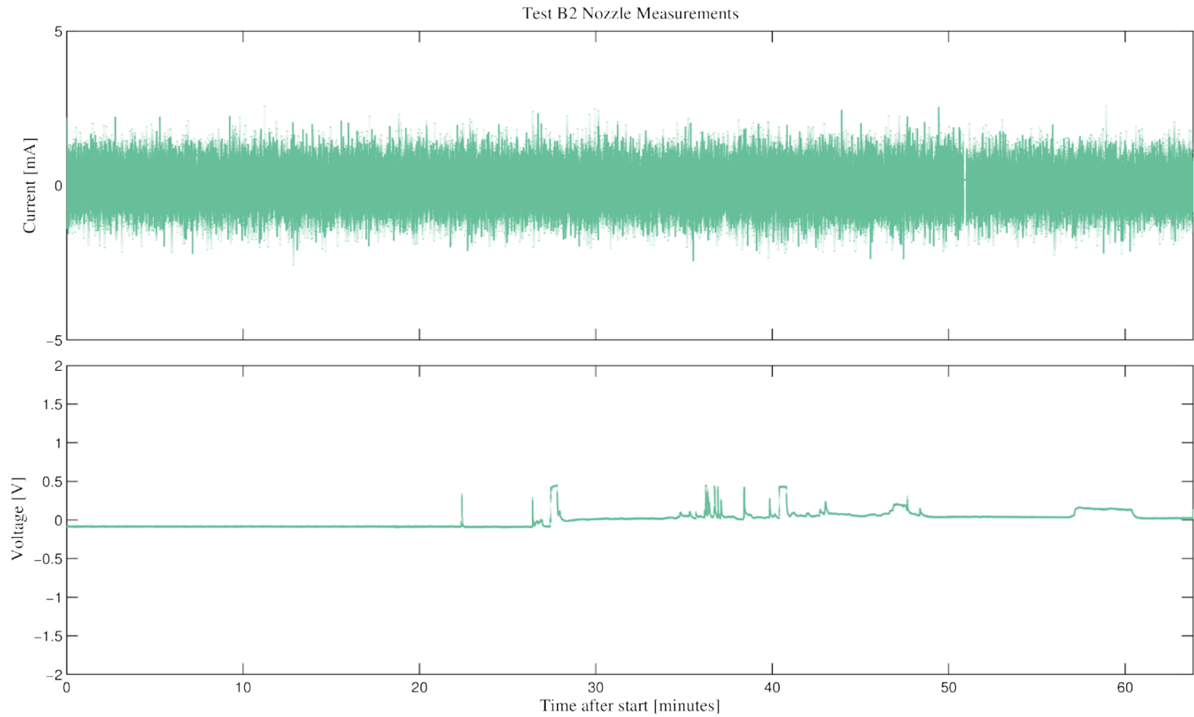
Figure E.7 Nozzle voltage and current measurements for Test B2
