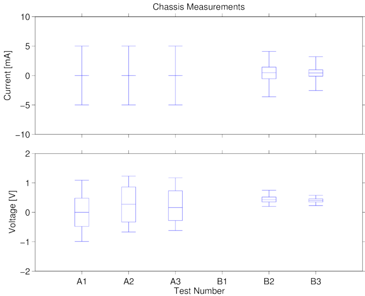
Figure E.2 Box plot indicating the maximum, minimum, median, first quartile and third quartile measurement for chassis voltage and current measurements
