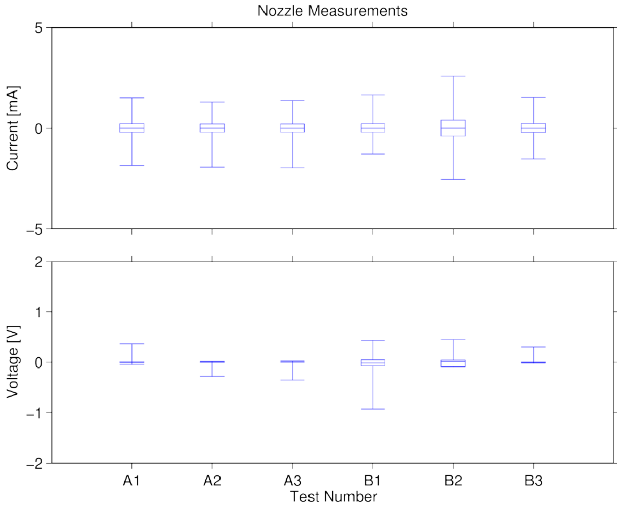
Figure E.1 Box plot indicating the maximum, minimum, median, first quartile and third quartile measurement for nozzle voltage and current measurements
