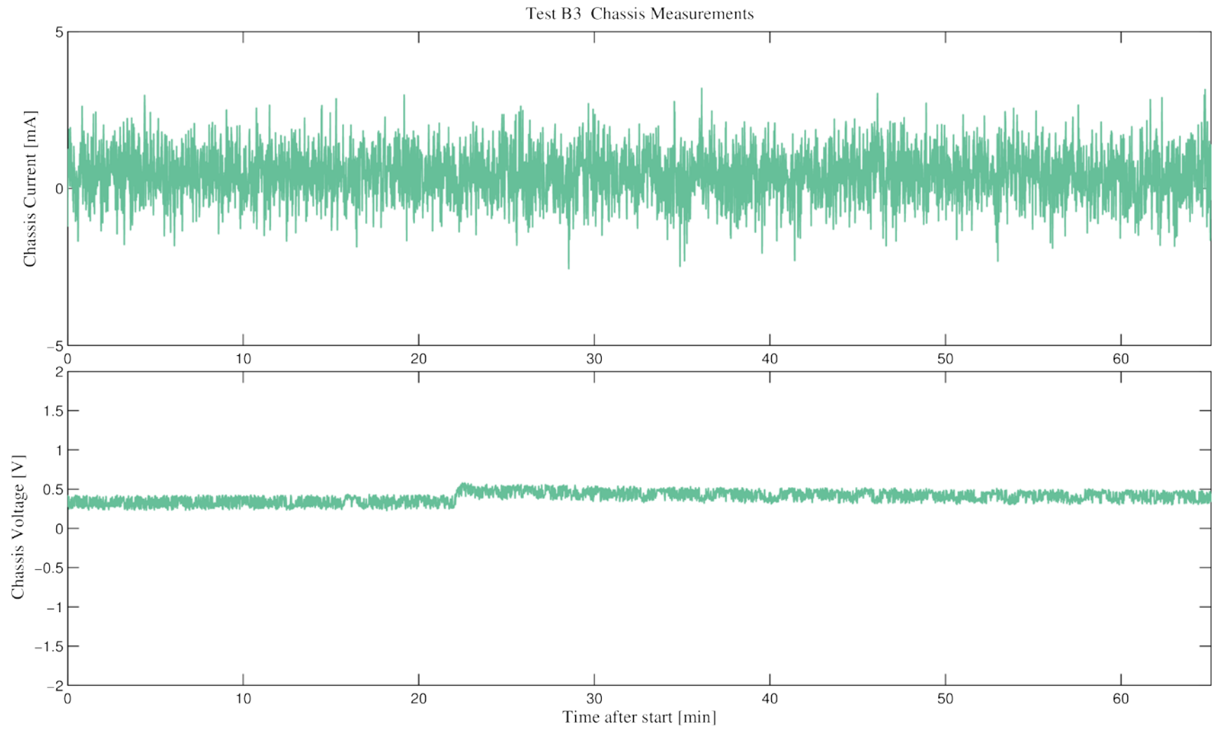
Figure E.14 Chassis voltage and current measurements for Test B3
