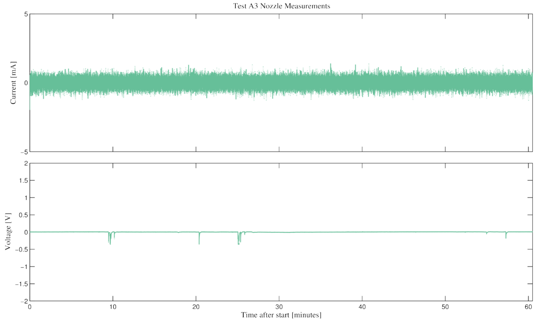
Figure E.5 Nozzle voltage and current measurements for Test A3
