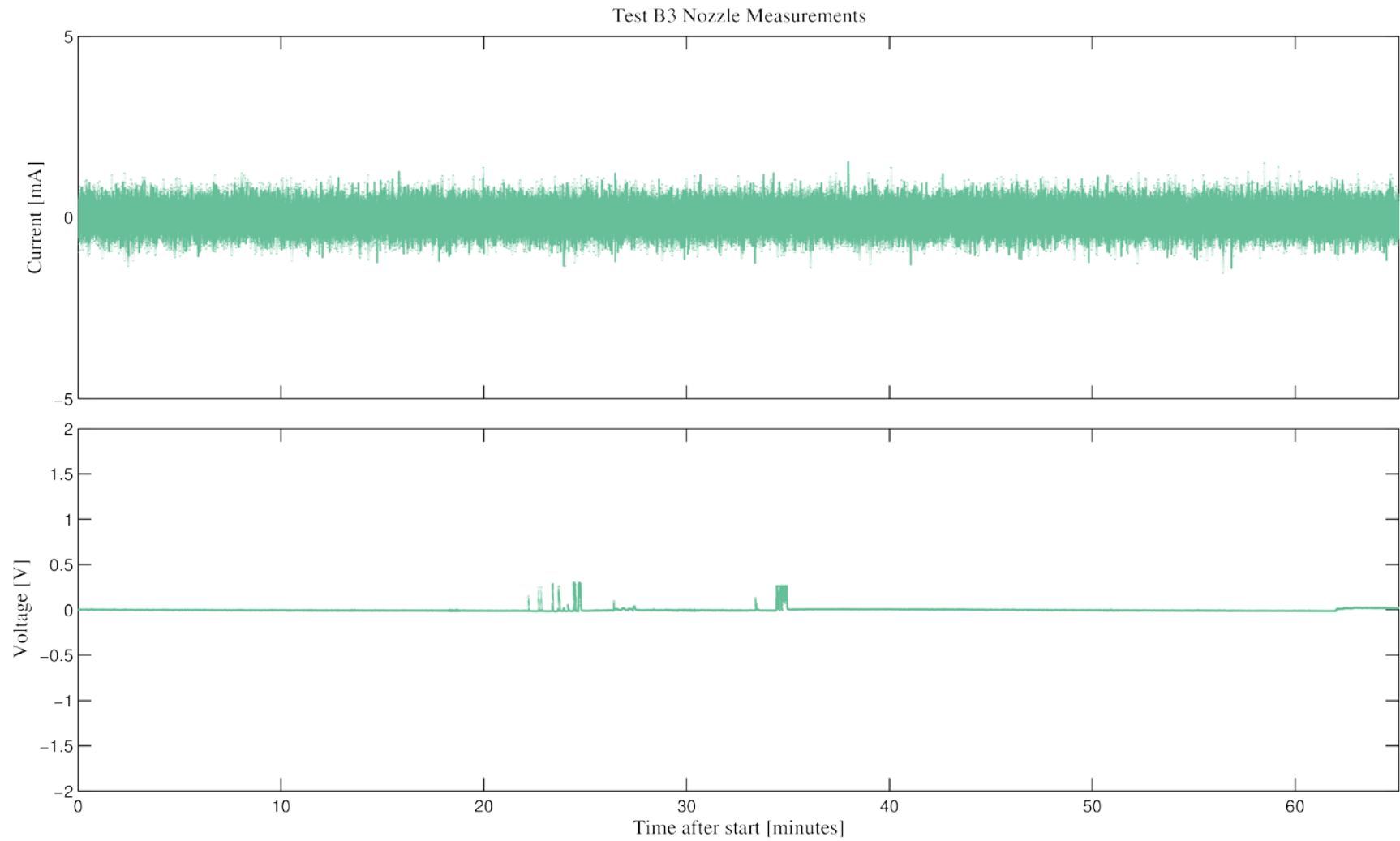
Figure E.8 Nozzle voltage and current measurements for Test B3
