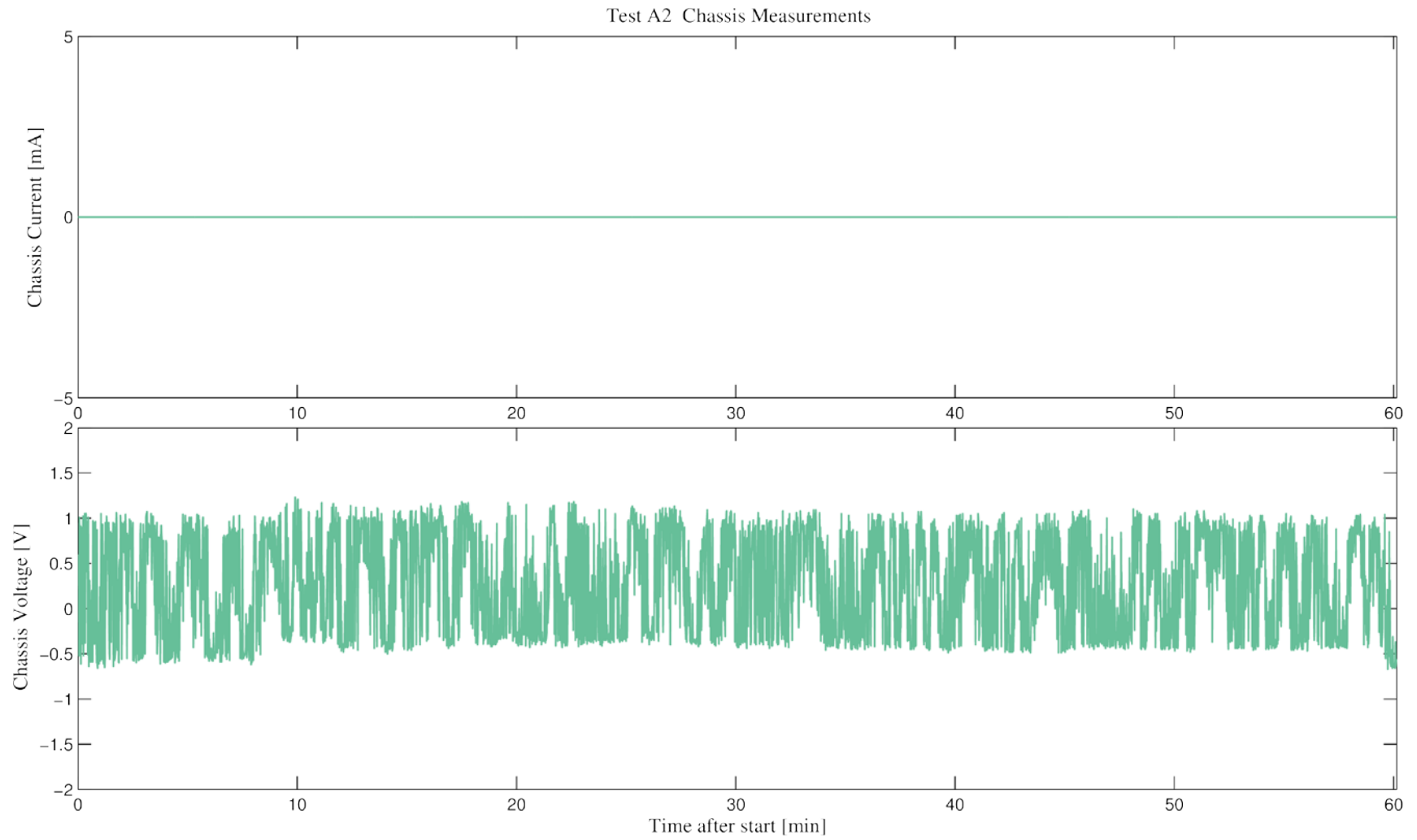
Figure E.10 Chassis voltage and current measurements for Test A2
