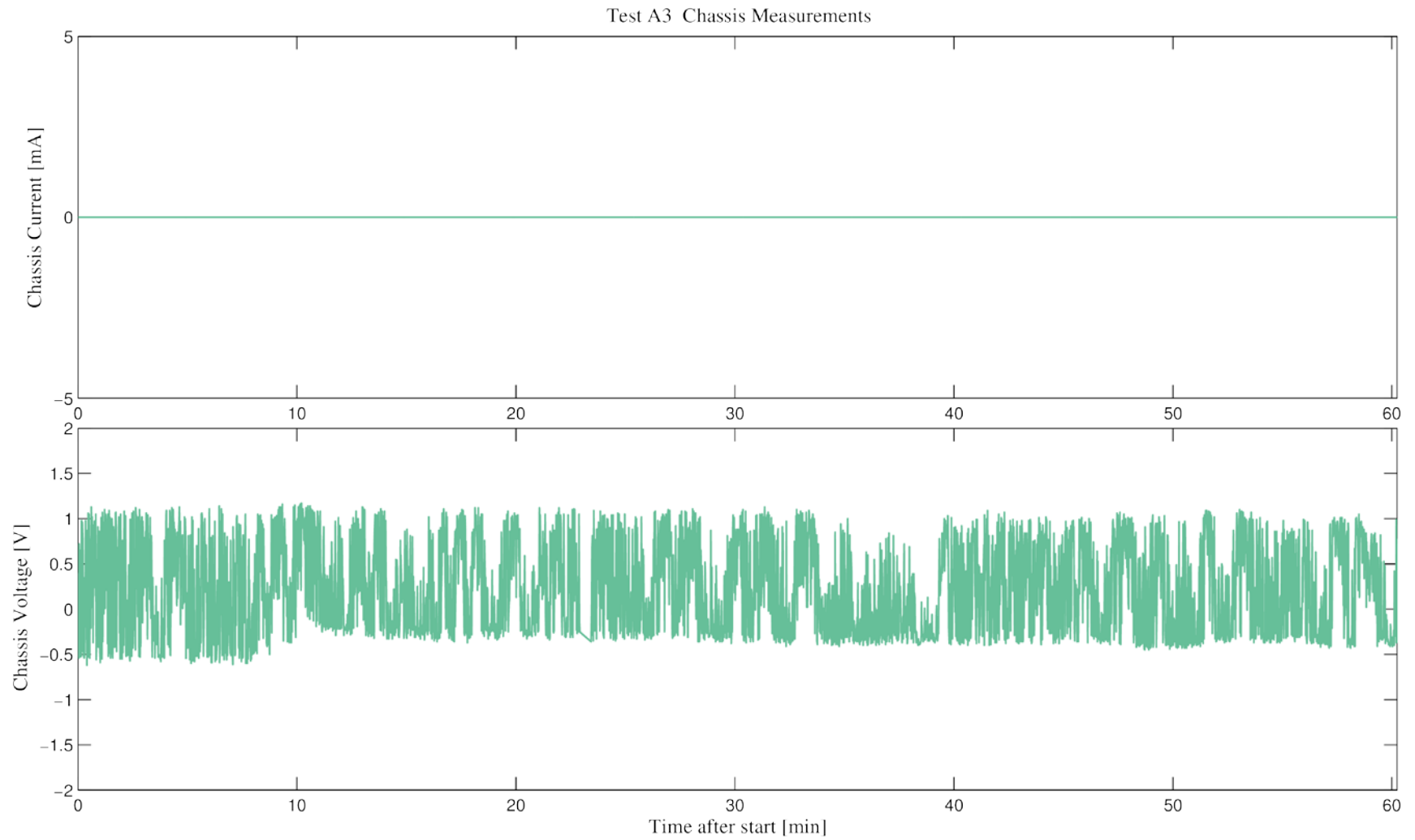
Figure E.11 Chassis voltage and current measurements for Test A3
