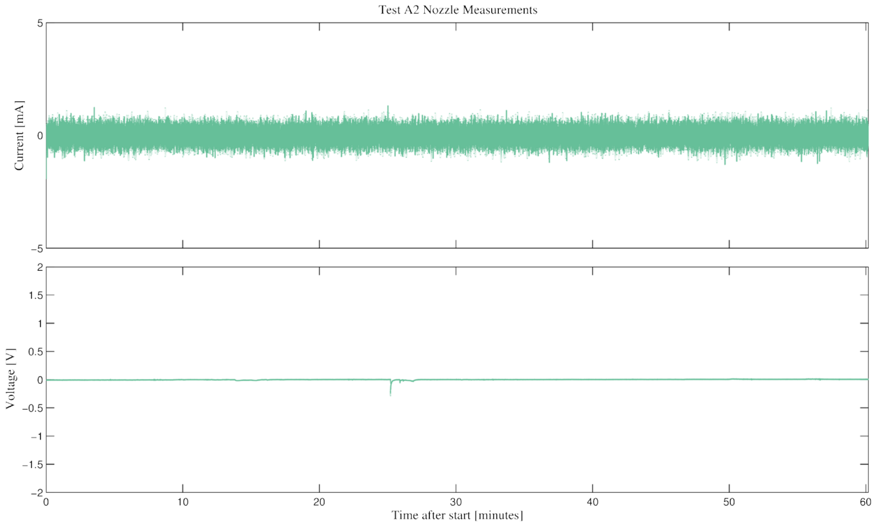
Figure E.4 Nozzle voltage and current measurements for Test A2
