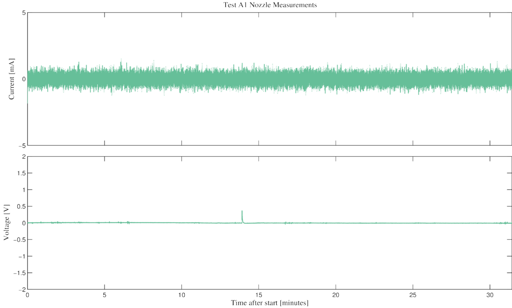
Figure E.3 Nozzle voltage and current measurements for Test A1
