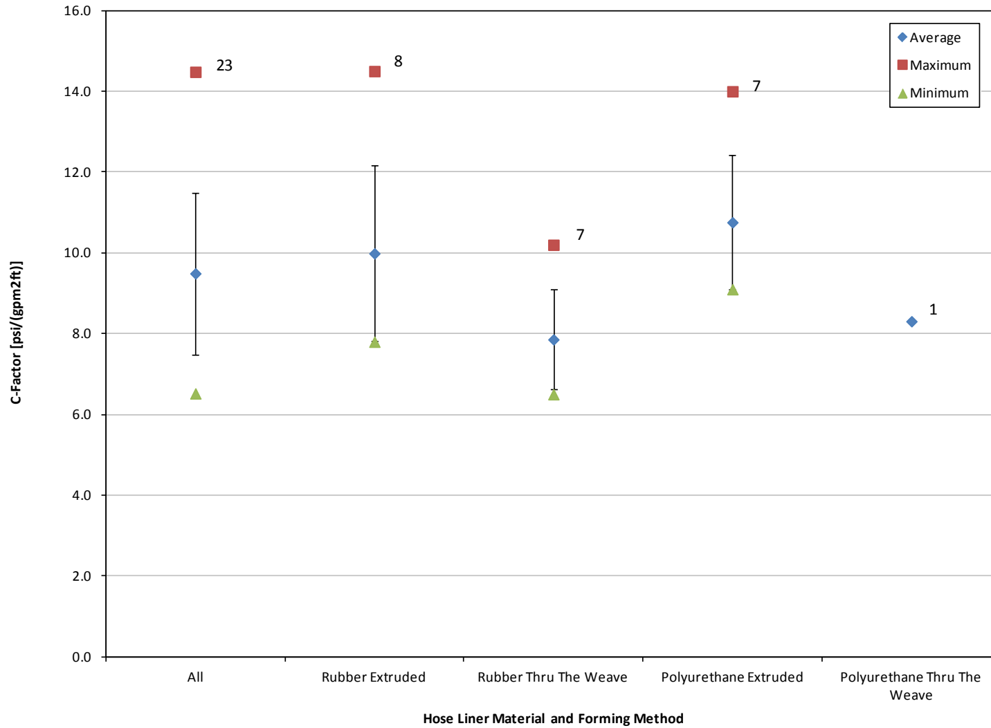
Figure D.3. Plot of Friction Loss Factor, C, by Hose Liner Material and Forming Method – 1.75-inch Hoses. Note: Error bars shown as the first standard deviation from the average. The number of tests is noted for each Hose Liner Material and Forming Method.
