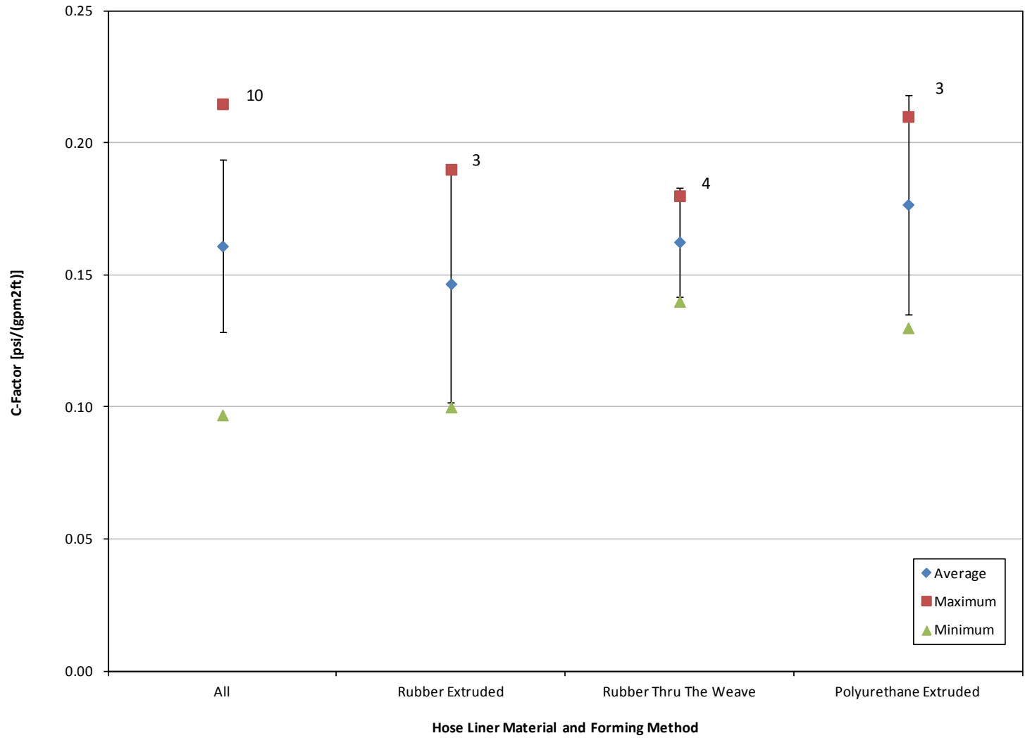
Figure D.5. Plot of Friction Loss Factor, C, by Hose Liner Material and Forming Method – 4-inch Hoses. Note: Error bars shown as the first standard deviation from the average. The number of tests is noted for each Hose Liner Material and Forming Method.
