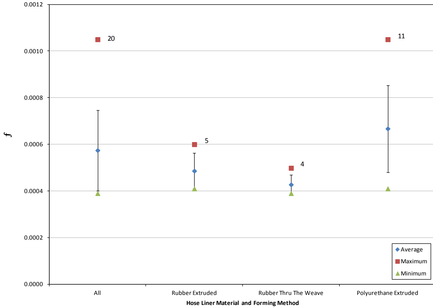
Figure C.3. Plot of Friction Loss Coefficient, f , by Hose Liner Material and Forming Method – 1.5 inch Hoses.
