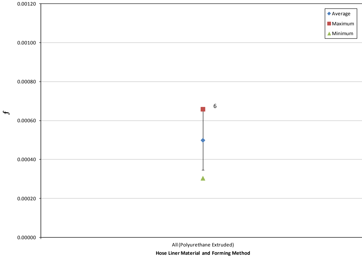
Figure C.2. Plot of Friction Loss Coefficient, f , by Hose Liner Material and Forming Method – 1.0 inch Hoses. Note: Error bars shown as the first standard deviation from the average. The number of tests is noted for each Hose Liner Material and Forming Method.
