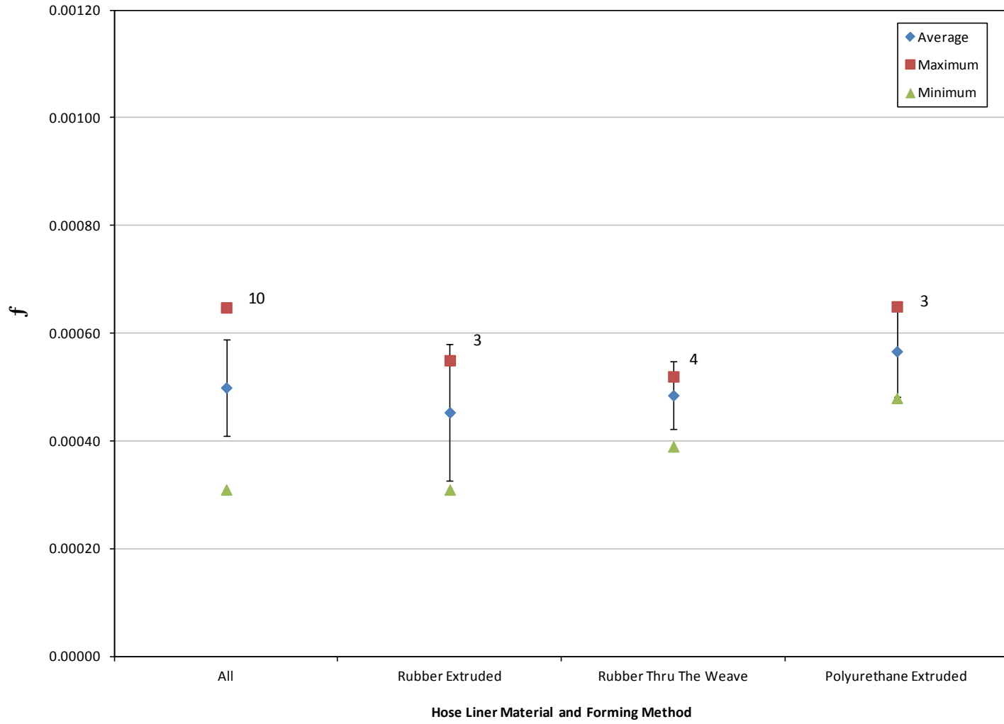
Figure C.6. Plot of Friction Loss Coefficient, f , by Hose Liner Material and Forming Method – 4 inch Hoses. Note: Error bars shown as the first standard deviation from the average. The number of tests is noted for each Hose Liner Material and Forming Method.
