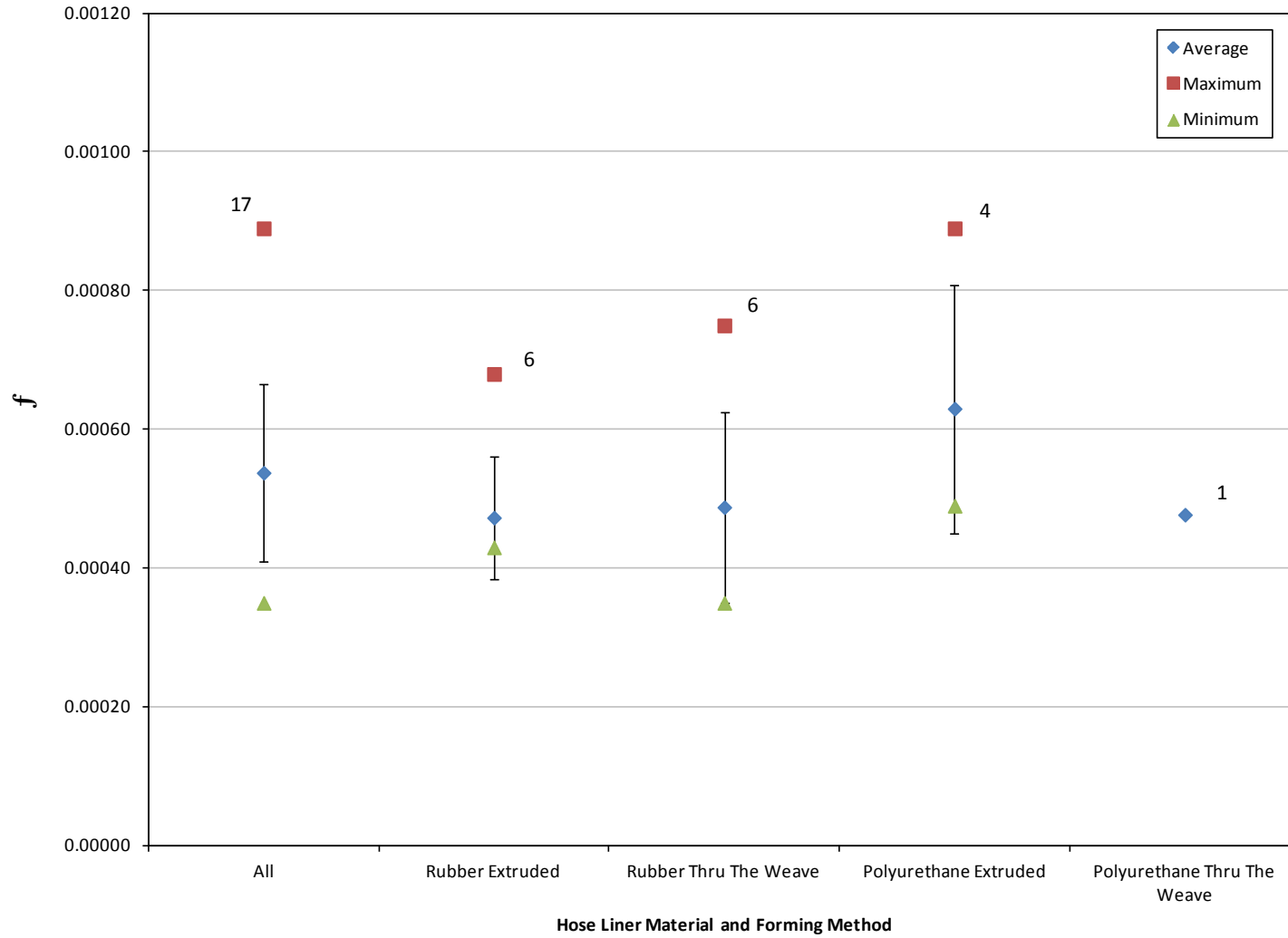
Figure C.5. Plot of Friction Loss Coefficient, f , by Hose Liner Material and Forming Method – 2.5 inch Hoses.
